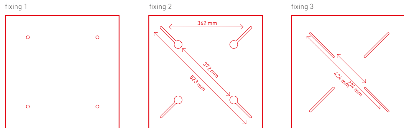
Installation of inserts for M6 screws.
